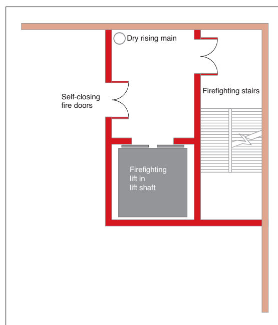
Figure 20: Firefighting shaft
