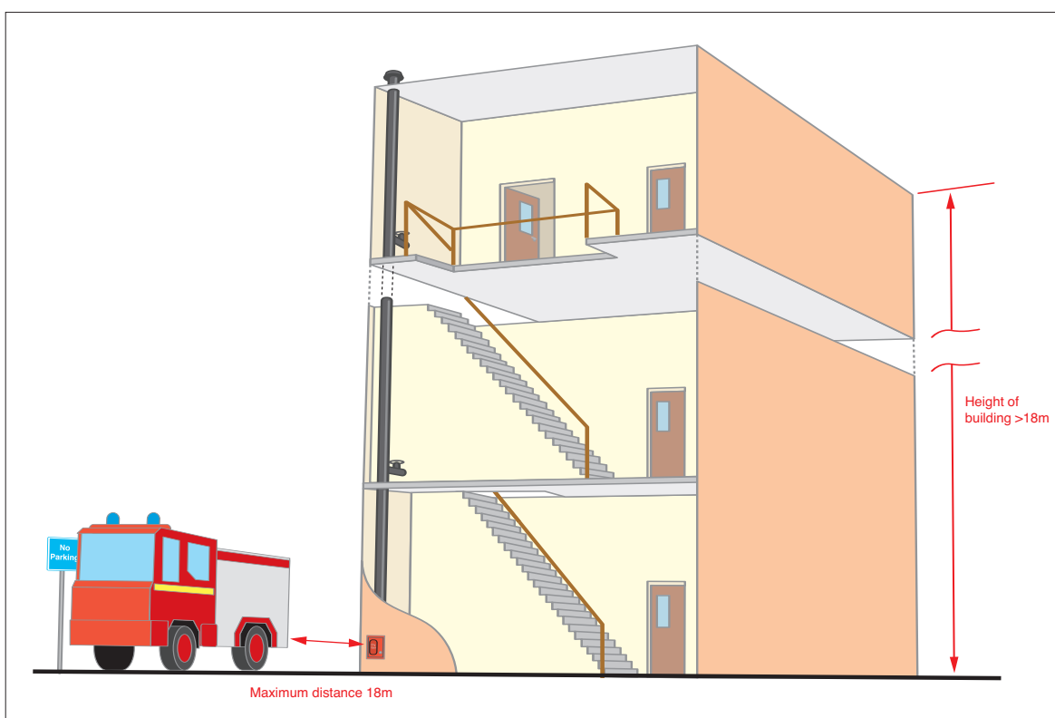
Figure 21: Rising main
